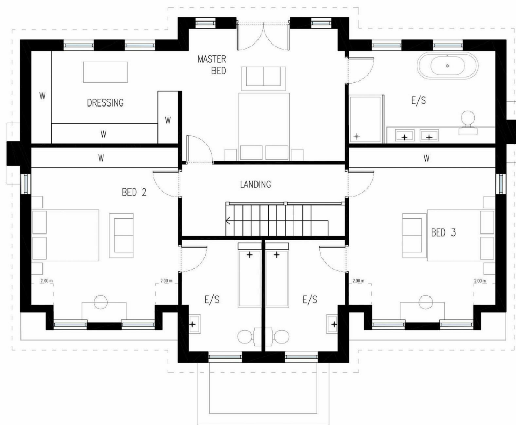
1ST FLOOR GIA FIRST FLOOR = 114 m 2
